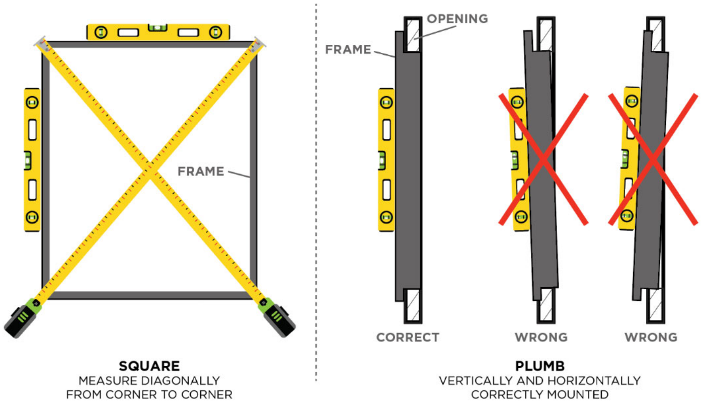
Figure 17.1: Frame Alignment, Squareness, and Plumb
