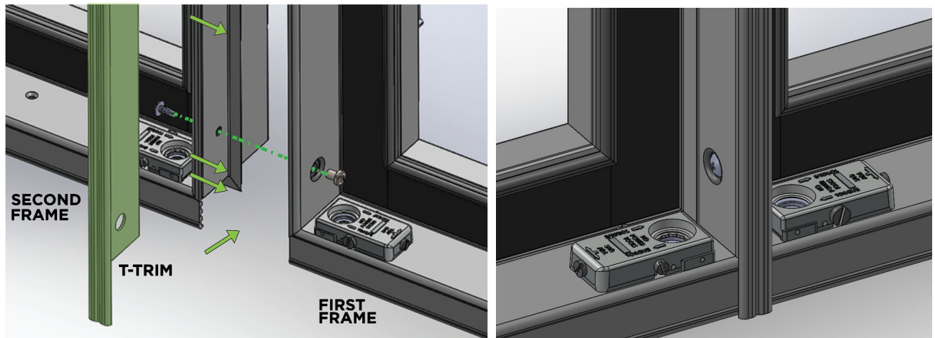
Figure 2.7: T-Trim installation
