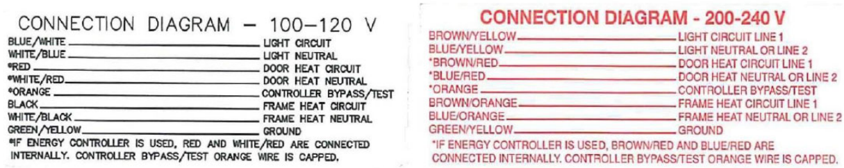
Figure 2.11: Wiring Labels
