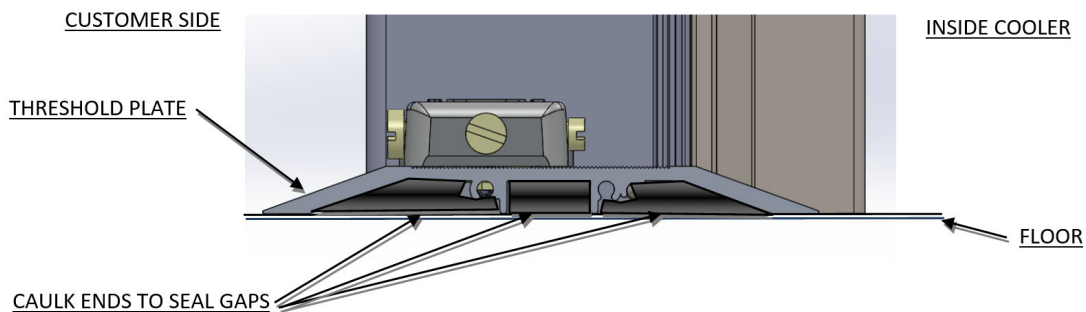
Figure 17.3: Sealing Threshold
