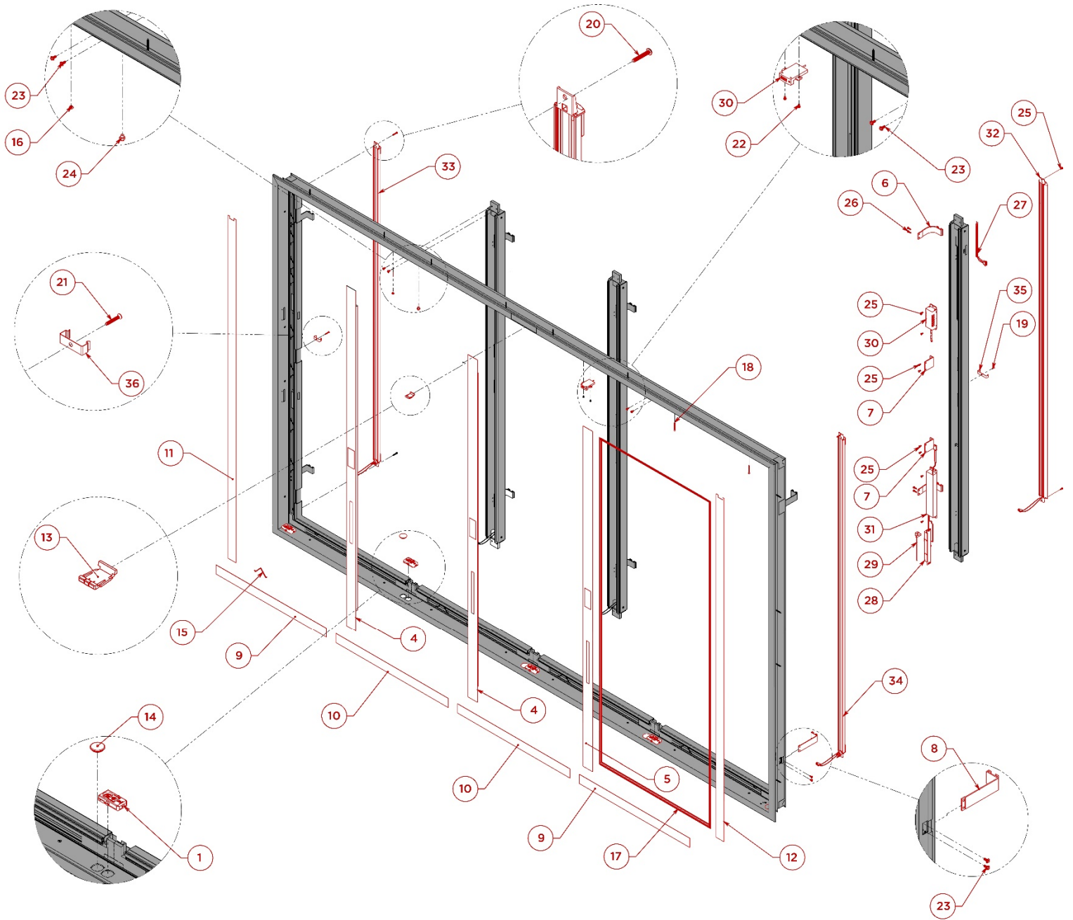
Figure 9.2 Frame Assembly for 101 Series Low Temperature for Replacement Parts (See Table 9.2 for part numbers)
