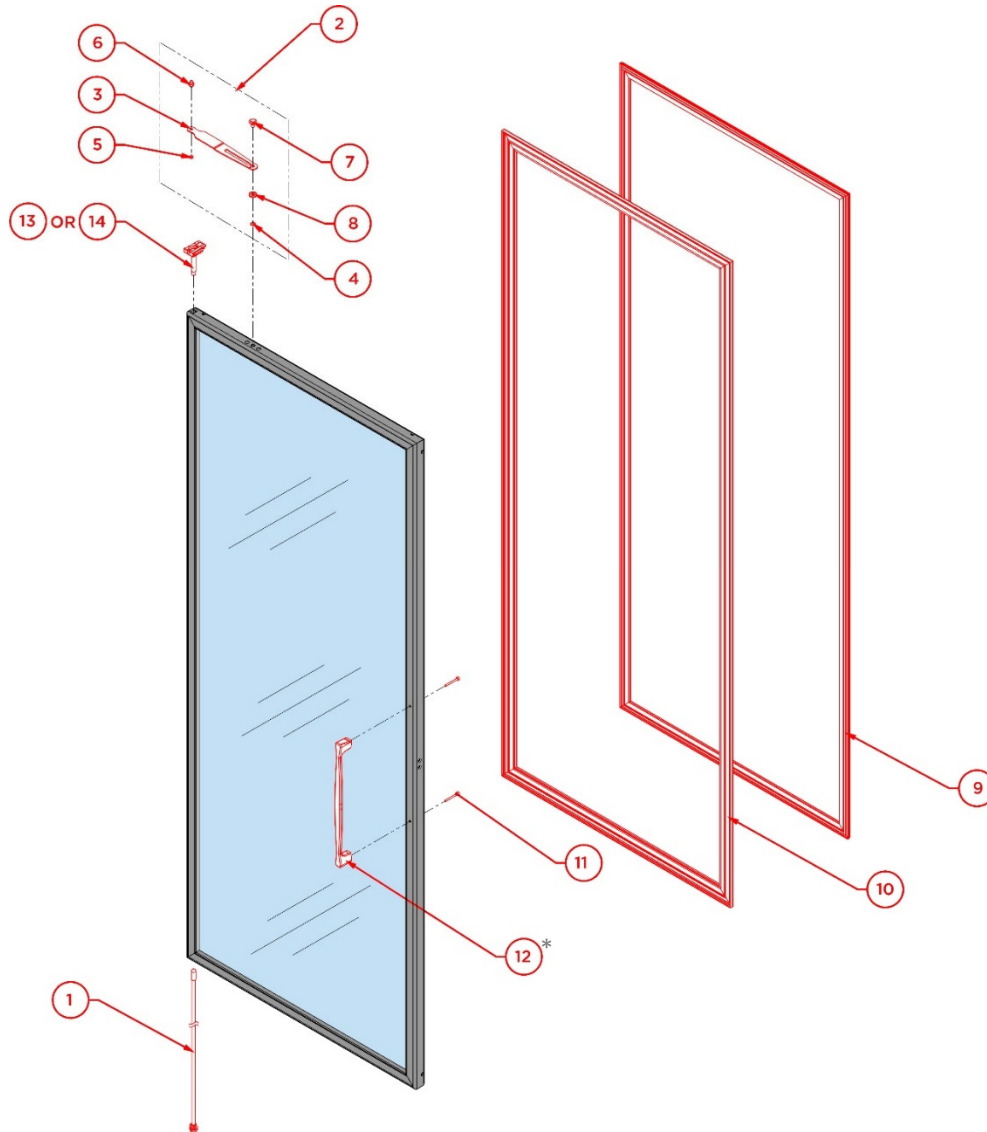
Figure 10.1 Door Assembly for 101 Series Door, for Replacement Parts
